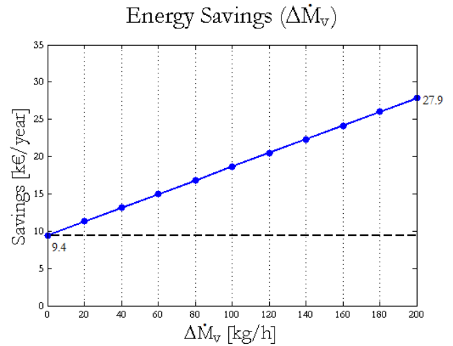
Figure 6: Energy savings as a function of steam rate variation.
