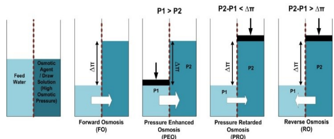
Figure 1: Possible processes based on osmosis ( http://ifoa.llobe.com/wp-content/uploads/2014/03/Osmotic_Processes_Diagram-1024x377.jpg )
