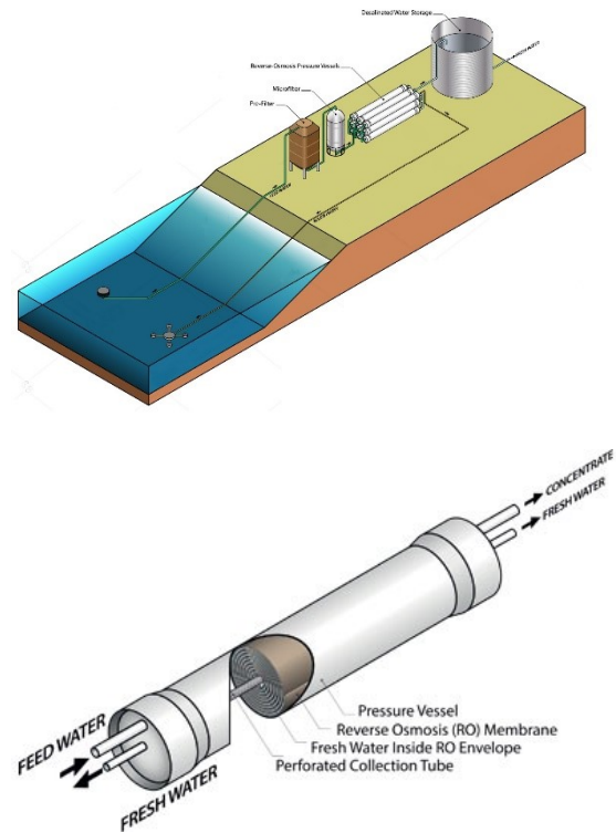
Figure 3: Osmosis water purification plant and detail of osmosis pressure vessel ( http://danolyte.com/it/progetti-speciali/desalinizzazione.html )
