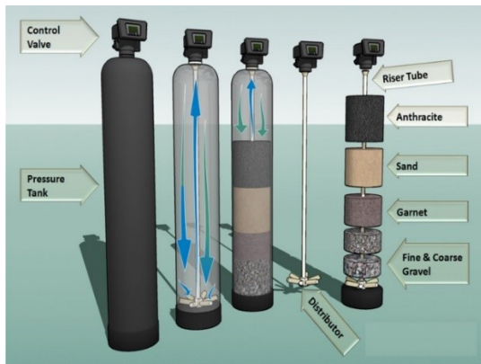
Figure 2: Example of mechanical multi-layer filter
